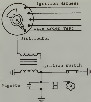
FIGURE 4-71. Breakdown not attributed to insulation failure.
